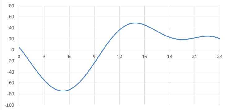
Gravity Tide at Shirahama (2016-10-09 JST in microGal)
